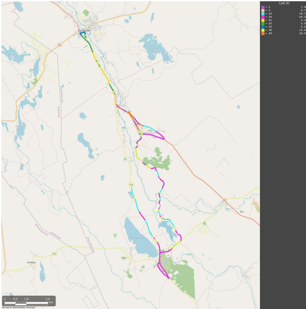
Cell ID
